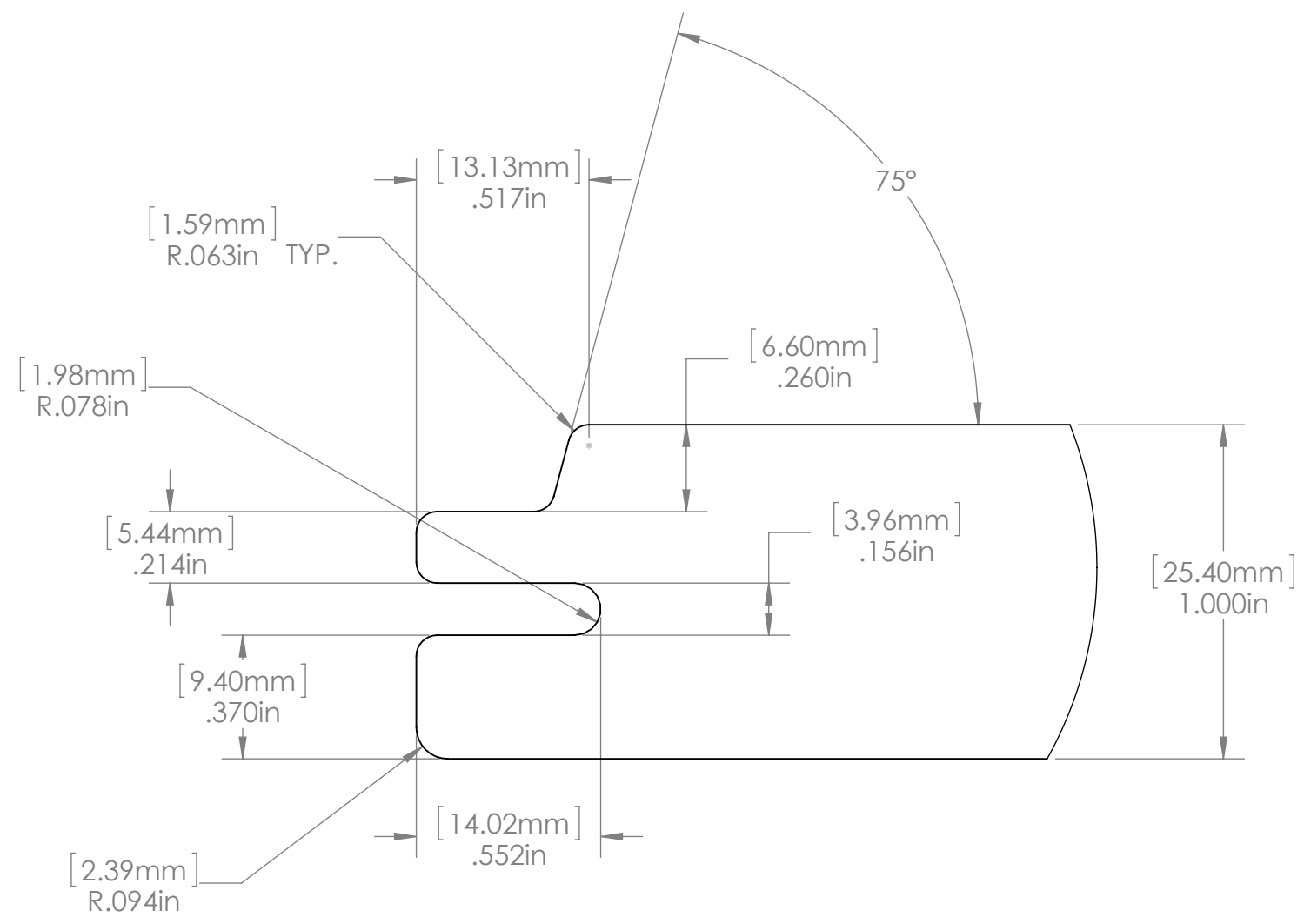
DETAIL B SCALE 2 : 1
